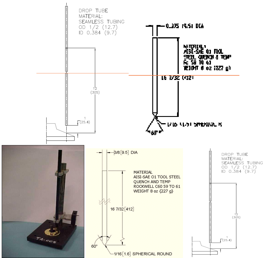
FIGURE 3—Projectile and Drop Tube
