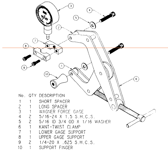
FIGURE 2 Thumbpiece-Test Fixture
