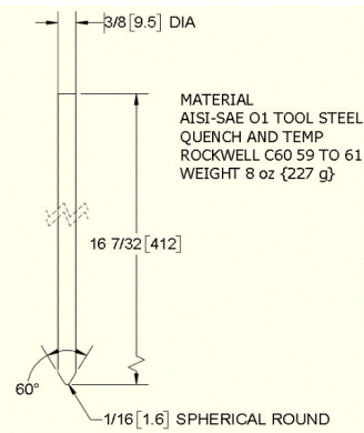
FIGURE 3 Projectile and Drop Tube
