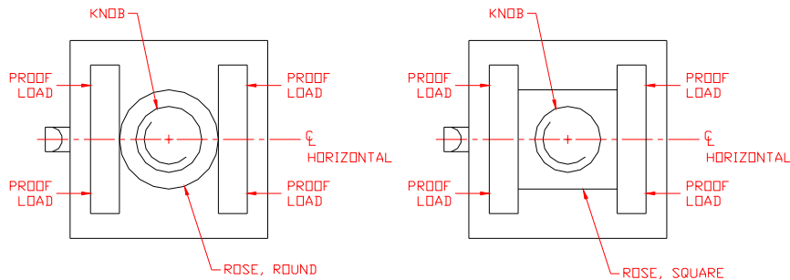
FIGURE 5-4 Outside Rose Deformation
